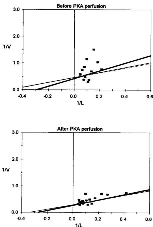
FIGURE 2 Plots of 1/v versus 1/L for a PKA experiment. Data points are from consolidation method I. Thick line shows fit from Levenberg-Marquardt-derived hyperbolas for nonconsolidated data (before PKA \chi^2 = 16.0 , n = 29 ; after \chi^2 = 40.9 , n = 44 ). Lines from consolidation methods I and II (thin line, broken line) are identical.
