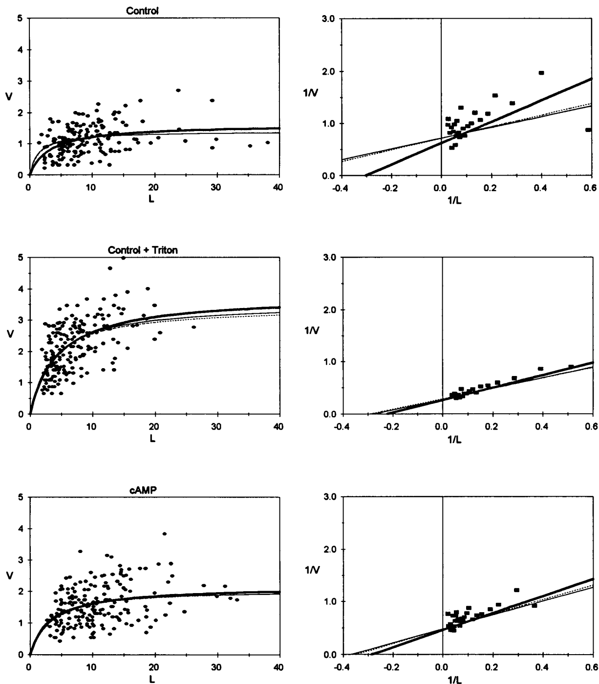
FIGURE 1 (a) Determination of v_0 and K_L by the Levenberg-Marquardt algorithm. The graphs show a typical data set to which optimal hyperbolas described by Eq. 3 have been fitted, so that values of a and b , representing v_0 and K_L , respectively, can be determined. The hyperbolas derived from data sets from consolidation methods I and II are also indicated in each instance. For the nonconsolidated data sets shown: control: \chi^2 converges to 34.0 ( n = 183 ); control + Triton: \chi^2 converges to 83.2 ( n = 205 ); cAMP: \chi^2 converges to 66.9 ( n = 204 ). (b) Plots of 1/v versus 1/L for the data sets from the Levenberg-Marquardt-derived hyperbolas shown in a . The lines are drawn using the values from each hyperbola. The squares are data points from consolidated method I for visualization of fit. Note that -1/K_L is approximately constant in all cases. Thick lines: nonconsolidated data set. Thin and dotted lines: consolidated data sets I and II, respectively.
